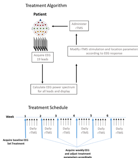
Fig. 1. Patient PrTMS treatment algorithm and the treatment schedule. Patient EEG recordings were acquired once every week for 4–6 weeks, in some cases longer, and the power spectrum derived from the EEG was used to determine what stimulation frequency and what cortical locations were treated. Patients received 5 daily treatments each week.
